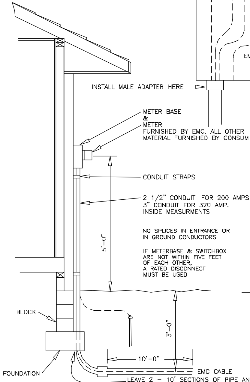
SIDE VIEW
